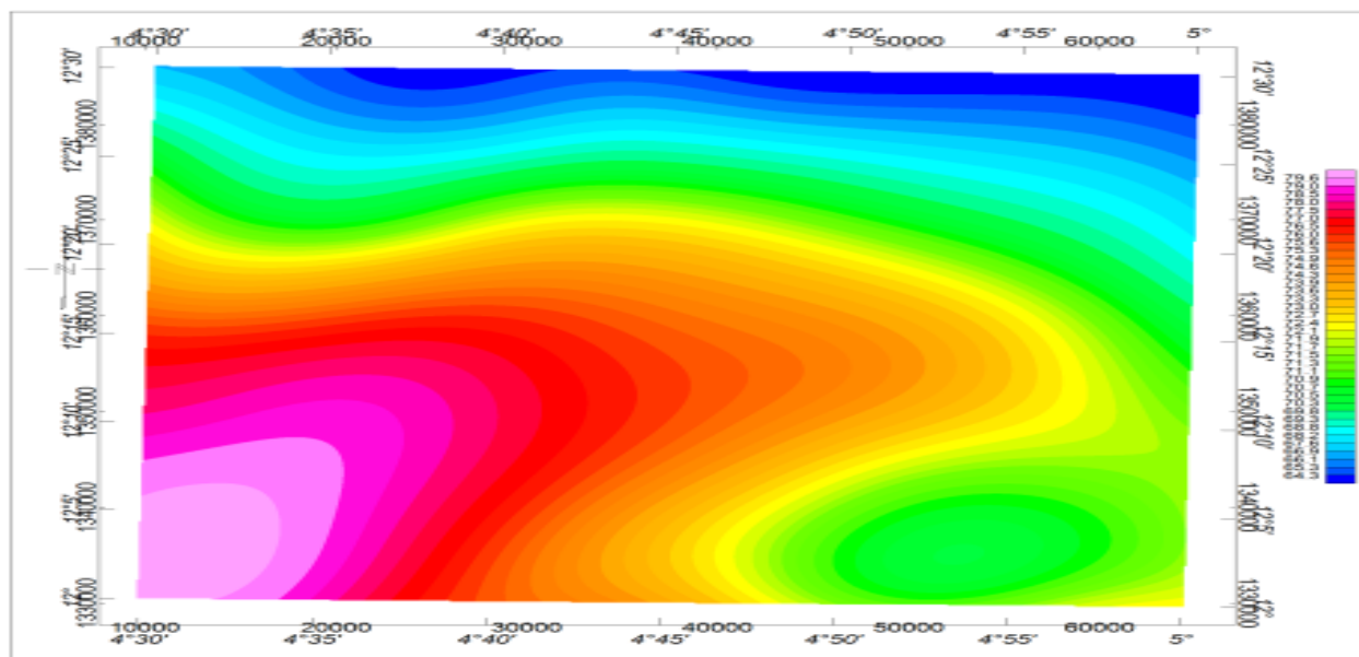
Figure 3.5 TMI at 10km
