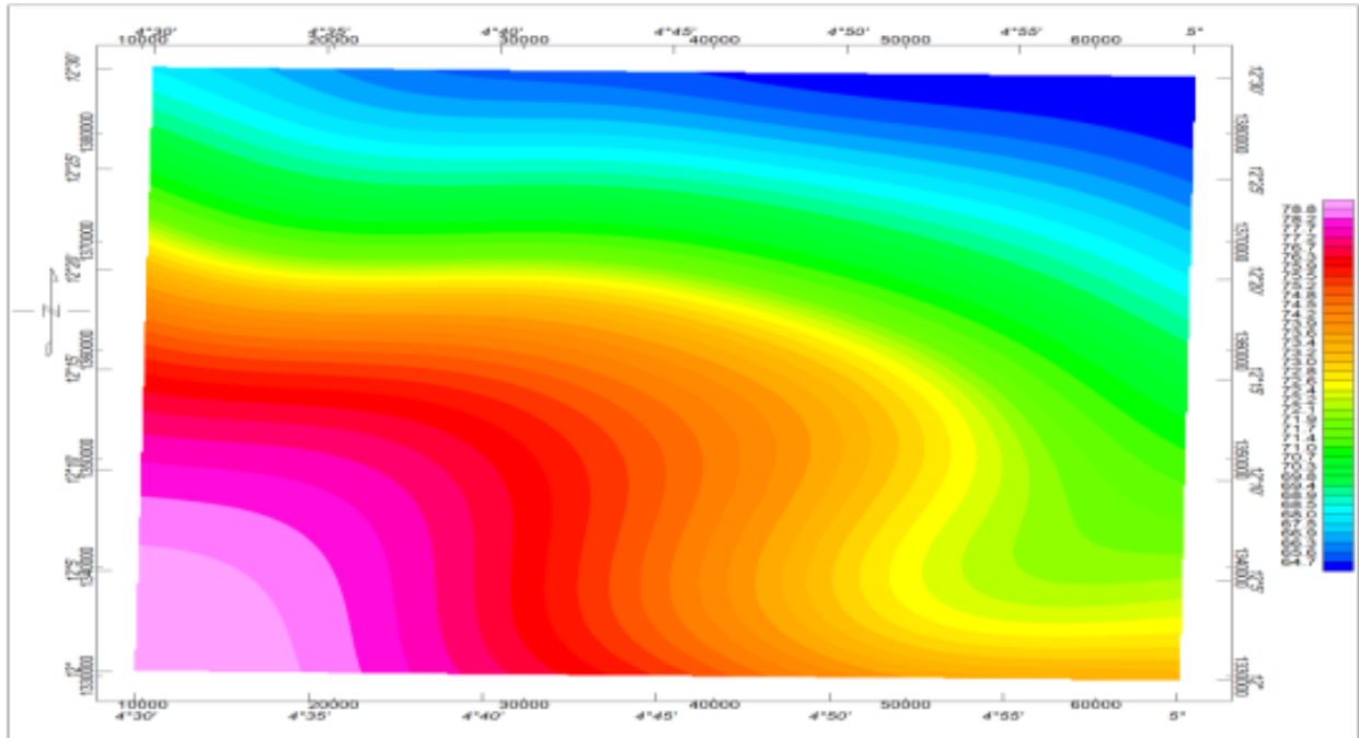
Figure 3.6 TMI at 15km
