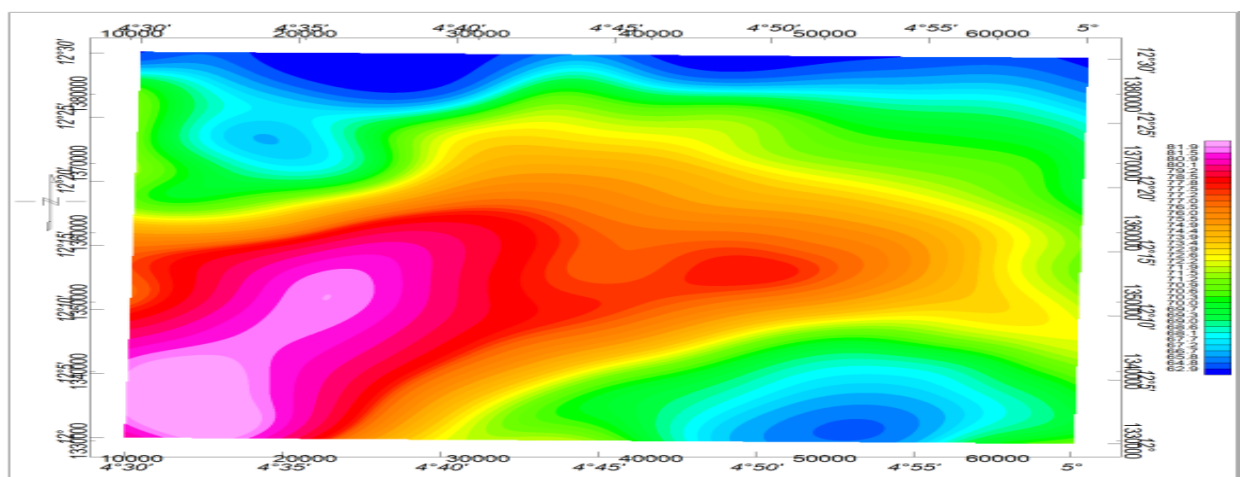
Figure 3.4 TMI at 5km
