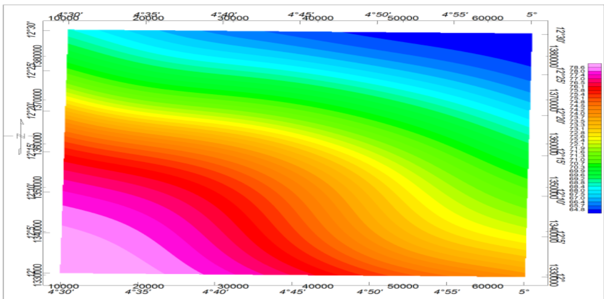
Figure 3.6 TMI at 20km
