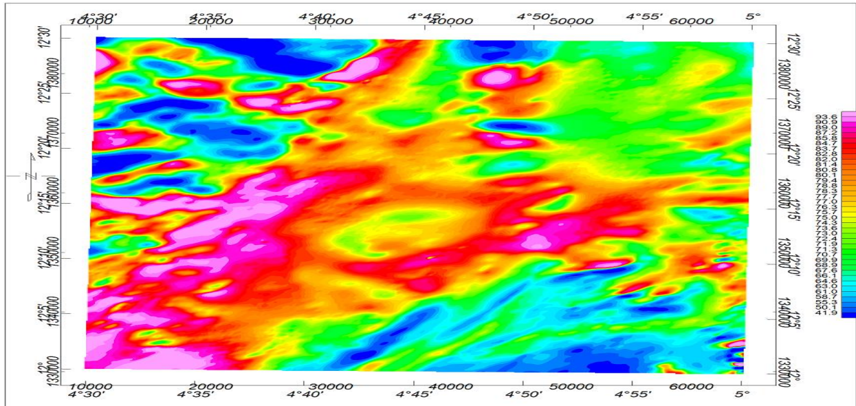
Figure 3.1 the total magnetic intensity map (TMI) of Tambuwal
