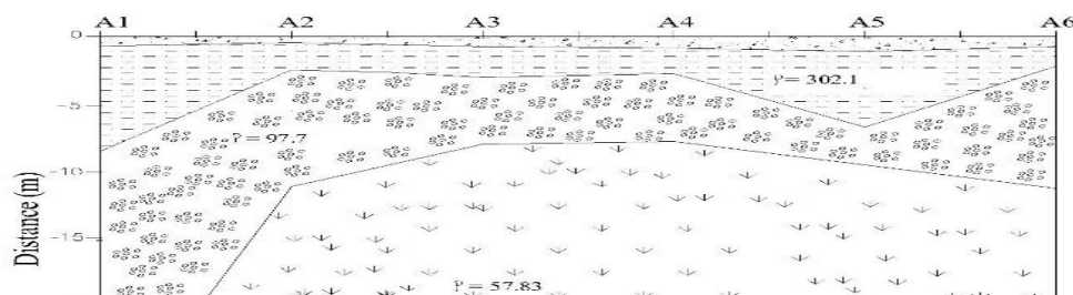
Figure 5a: Vertical Geo-electric Section of Profile A (Contour interval is 50 \Omega m)
