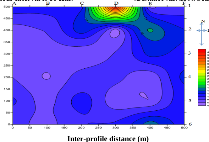
Figure 13: Iso-resistivity contour Map at 10 m depth (Distance (m) x 10) (Contour interval is 10 \Omega m)
