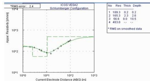
Figure 4b: Digitized WinResist Curve for VES A2. The curve type is H type is QH
