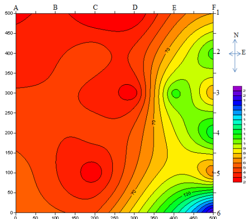
Figure 13: Iso-resistivity contour Map at 10 m depth (Distance (m) x 10) (Contour interval is 10 \Omega m)
