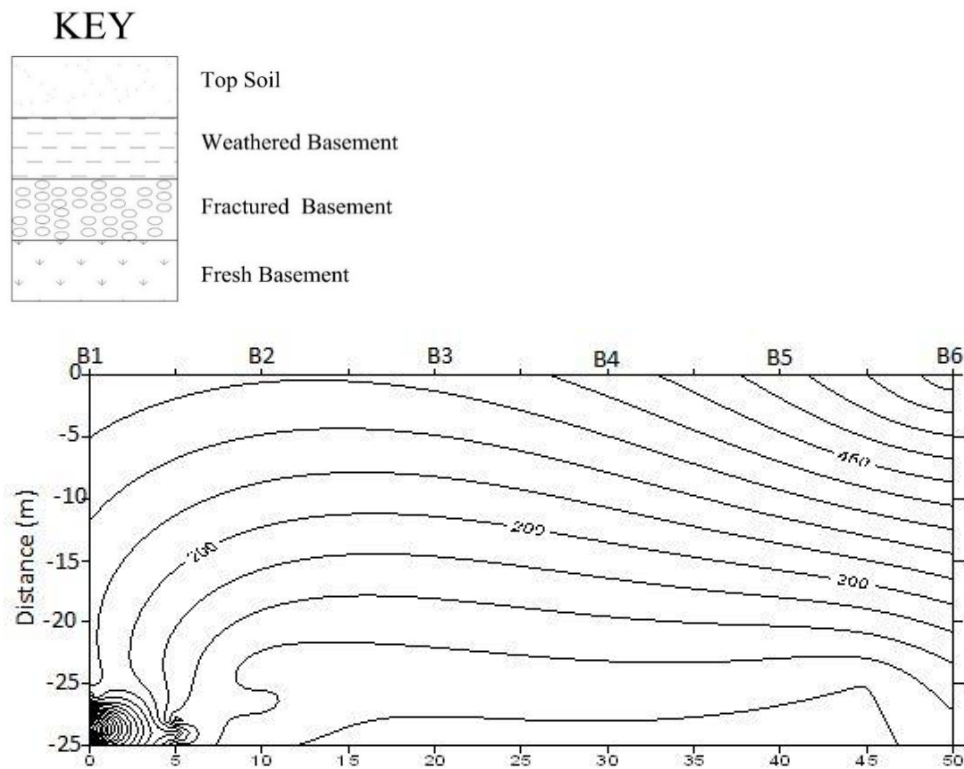
Figure 6a: Vertical Geo-electric Section of Profile B Distance (m) x 10(Contour interval is 50 Ωm)
