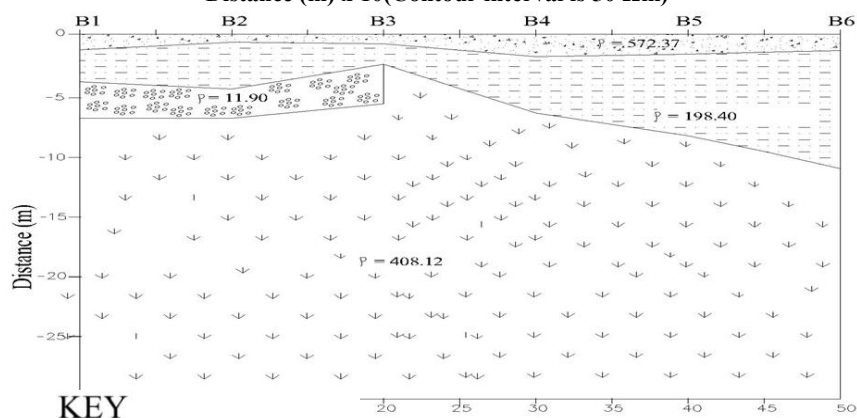
Figure 6b: Vertical Geo-electric Section of Profile B Distance (m) x10
