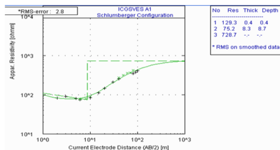
Figure 4a: Digitized WinResist Curve for VES A1.
