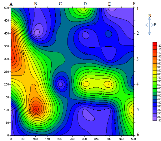
Figure 11: Iso-resistivity Contour Map at 1m depth (Distance (m) x 10) (Contour interval is 20 \Omega m) Distance (m) x 10) (Contour interval is 20 \Omega m)
