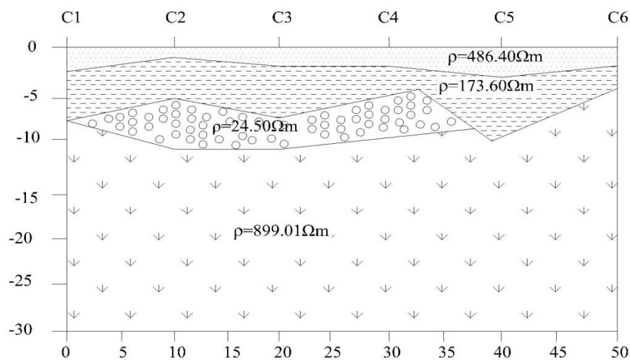
Figure 7b: Vertical Geologic Section of Profile C Distance (m) x 10)
