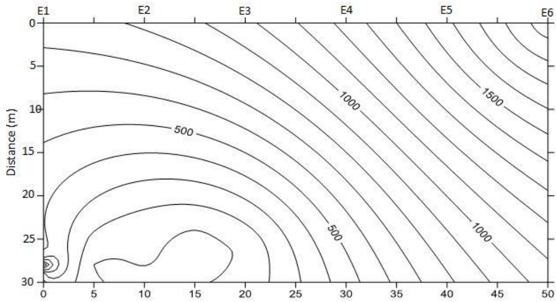
Figure 9a: Vertical Geo-electric Section of Profile E (Contour Interval is 100 \Omega m)
