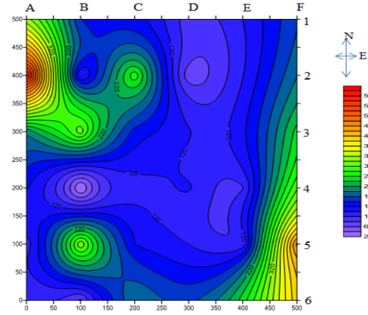
Figure 12: Iso-resistivity Contour Map at 5m depth
