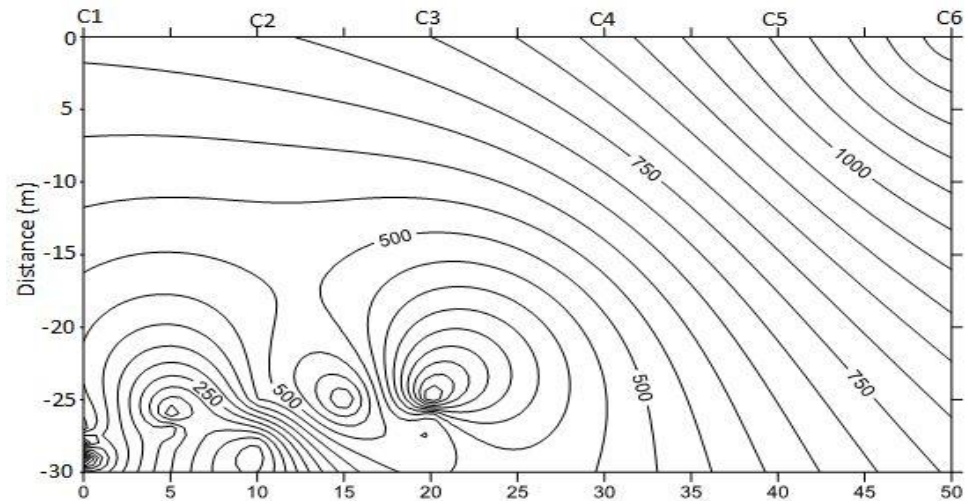
Figure 7a: Vertical Geo-electric Section of Profile C (Contour interval is 50 \Omega\text{m} )
