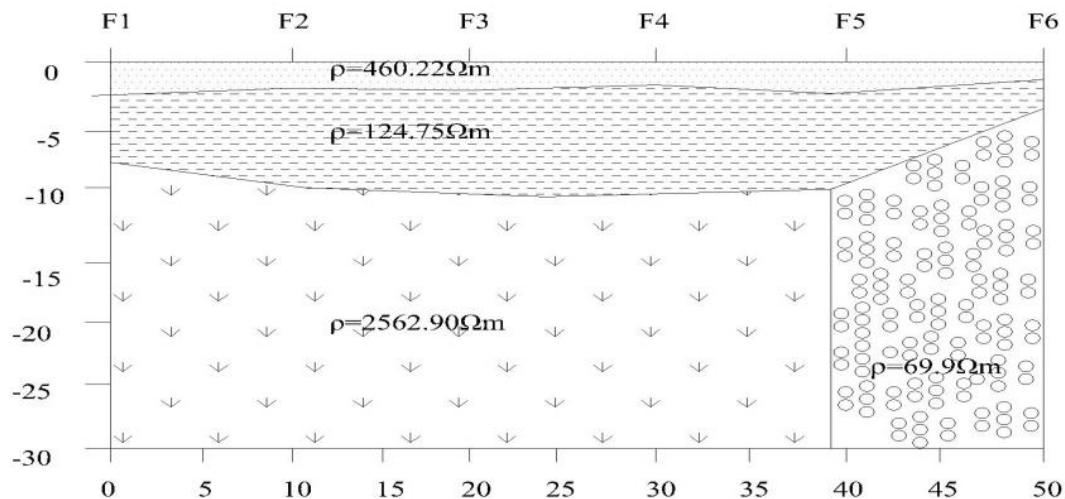
Figure 10b: Vertical Geologic Section of Profile F. Distance (m) x 10
