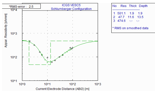
Figure 4c: Digitized WinResist Curve for VES A6. The curve type is KH
