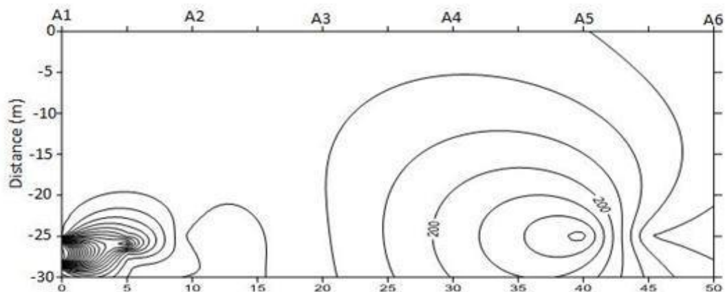
Figure 5a: Vertical Geo-electric Section of Profile A (Contour interval is 50 \Omega m)
