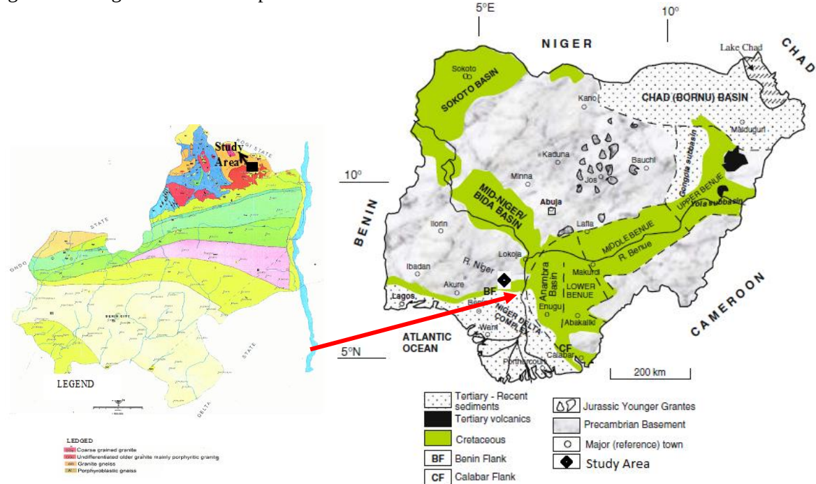
Figure2: Detailed geological map of Edo State culled from the Nigerian Geological Map (Obaje, 2009)
