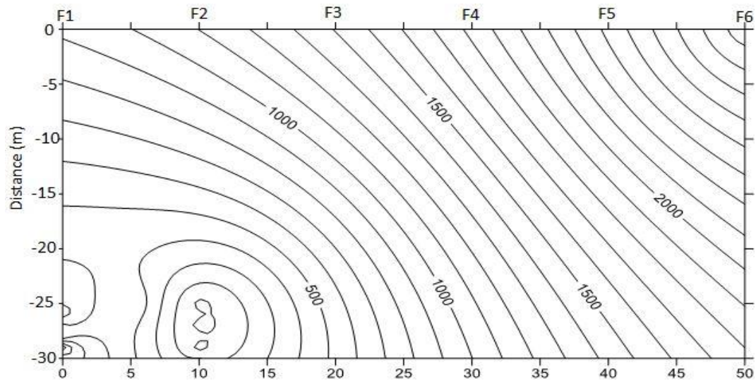
Figure 10a: Vertical geo-electric Section of Profile F (Contour Interval is 100 \Omega\text{m} )
